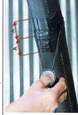
2. PVC tape; A = min. 15 cm.
