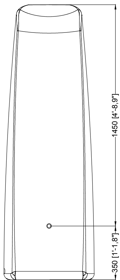
Vorderansicht View from front Vista frontal Vue de face
