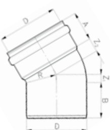
Koleno 30°
